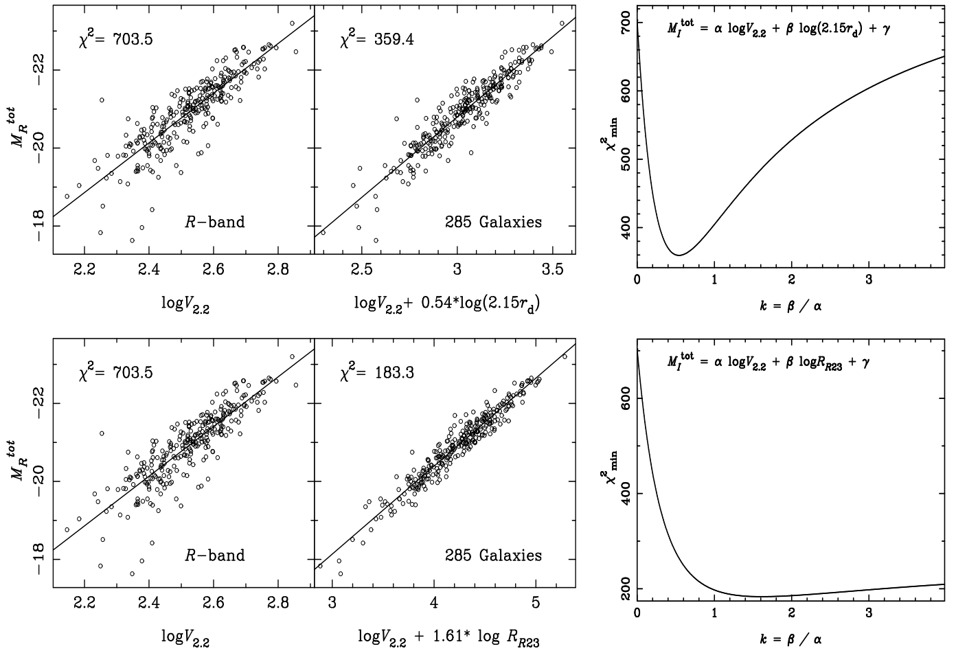
Fig. 4. Comparison of the Tully–Fisher relation (the left side) and the best plane (the right side). Data of 285 galaxies were taken from Courteau (1996,1997). The typical rms errors of the absolute magnitudes were taken as 0.3 mag. The variation in the fitting residual \chi^2 with the ratio k = \beta/\alpha is plotted on the right side.
